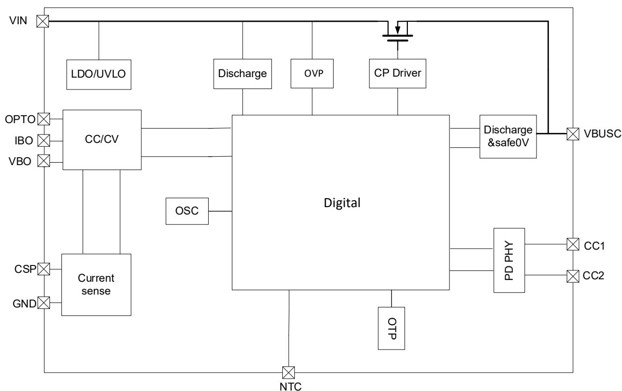
Fig. 3. Function Block
