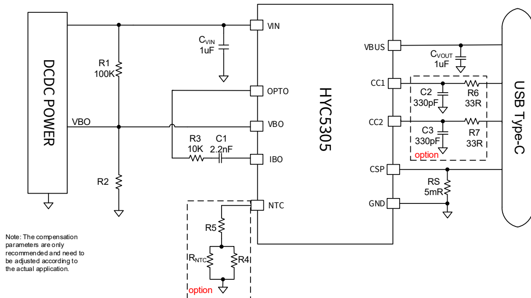
Fig. 7. Application for DCDC
