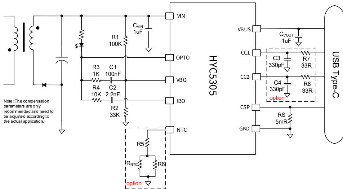
Fig. 6. Application for ACDC
