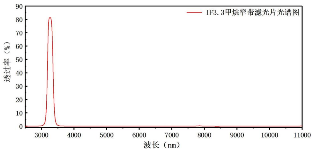
Transmittance of 3.30 \mu\text{m} Filter
