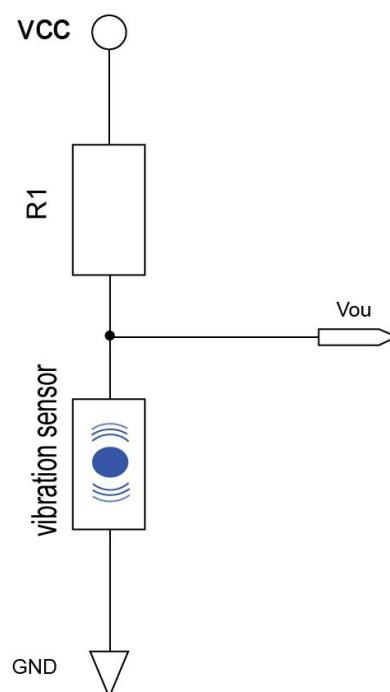
Figure 3: Basic circuit
