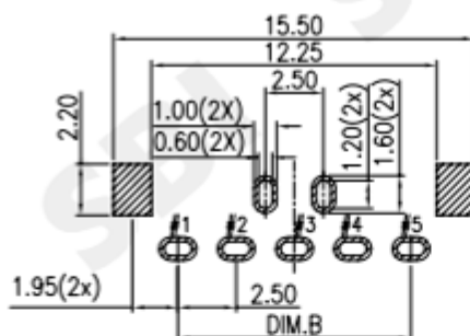
RECOMMENDED P.C.B LAYOUT TOP VIEW (TOLRANCE:±0.05)
