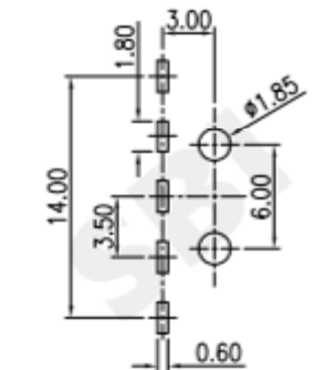
RECOMMENDED P.C.B LAYOUT TOP VIEW (TOLRANCE:±0.05) 3P/5P
