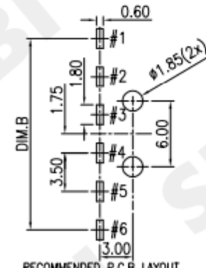
RECOMMENDED P.C.B LAYOUT TOP VIEW (TOLRANCE:±0.05) 4P/6P
