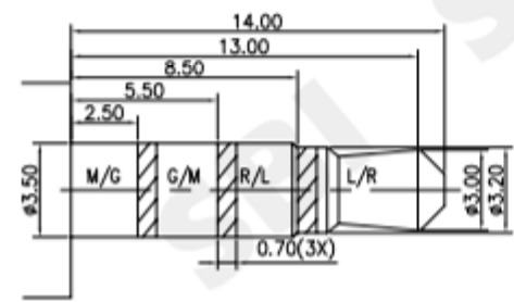
MATING PLUG
